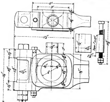
Figs. 1211-1217. Crank Pin Stub End of Main Rod for Consolidation (2-8-0) Locomotive. American Locomotive Co.
